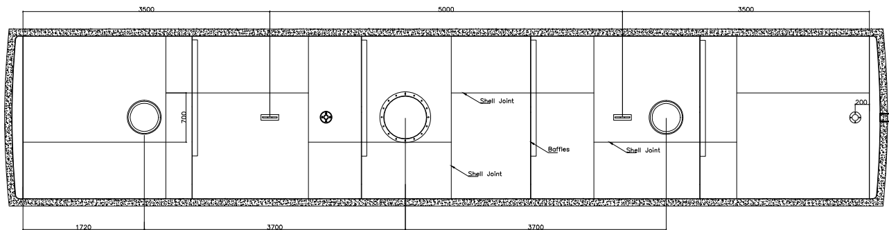
TOP VIEW
