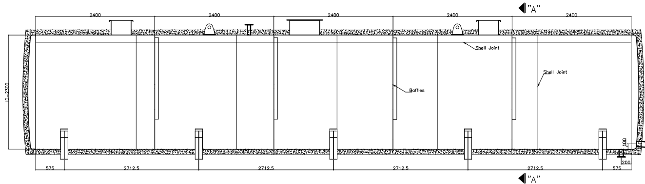
FRONT VIEW
